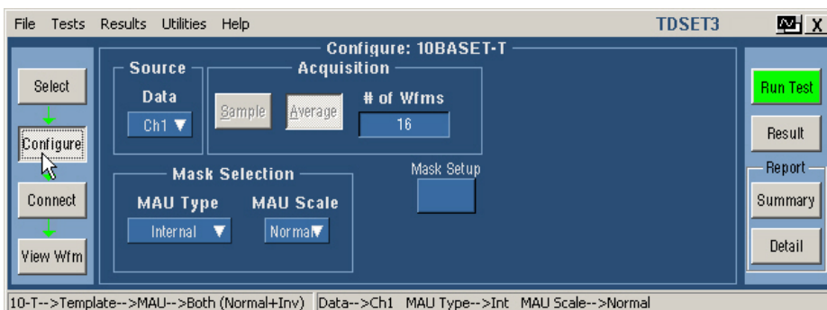
Figure 5- 3: 10BASE-T Configure pane
