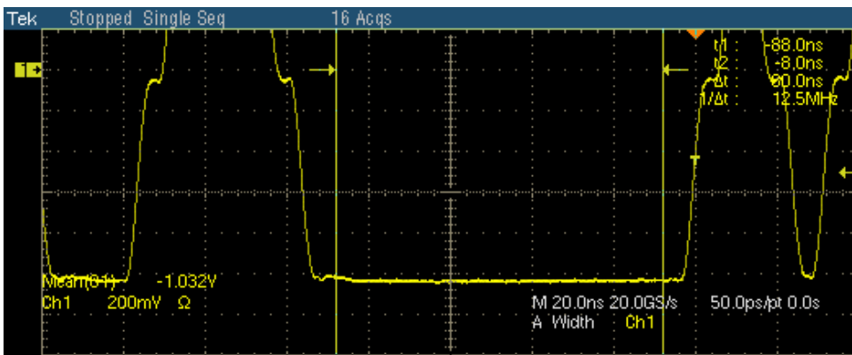
Figure 9-8: Waveform for 100BASE-TX Rise Time for Negative polarity
