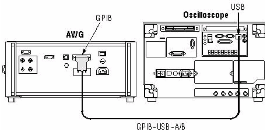
Figure 15-2: Connecting the AWG and the Oscilloscope
