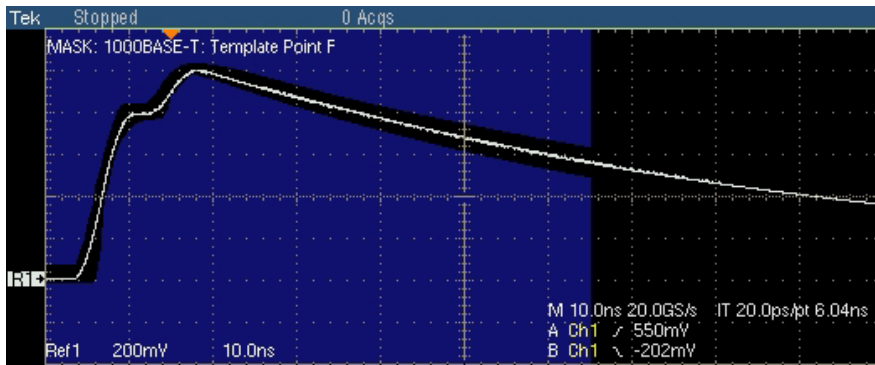
Figure 8-2: Waveform for 1000BASE-T Template Points F and H
