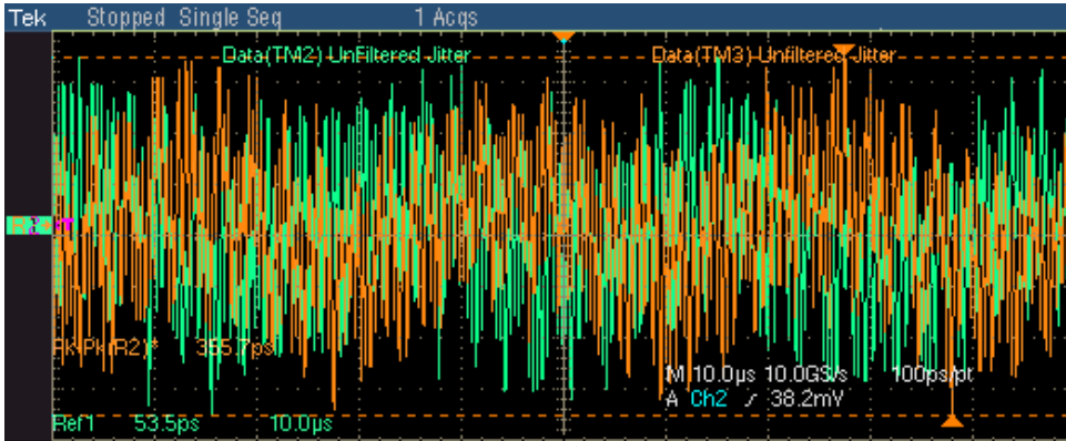
Figure 8-19: TIE Waveform for 100BASE-T Jitter Slave Unfiltered
