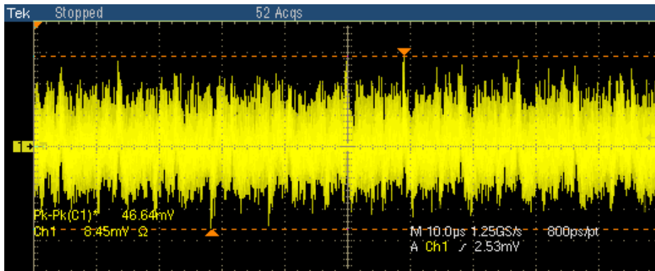
Figure 8-24: Waveform for 1000BASE-T Common mode Voltage
