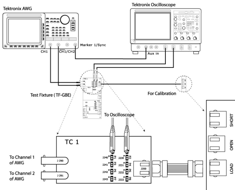
Figure 18-1: Calibration for 1000BASE-T Return Loss
