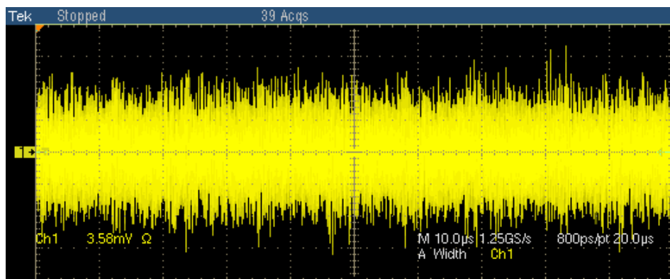
Figure 10-25: Waveform for 10BASE-T Common mode Voltage
