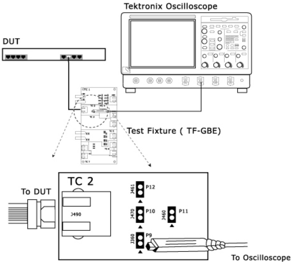
Figure 3-28: Step 1 Connections of Test Fixture Compensation
