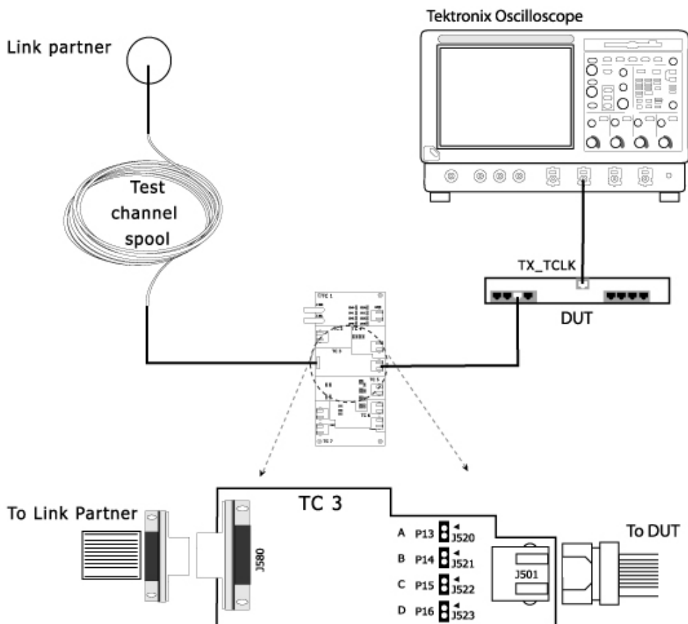
Figure 6-6: 100BASE-T Connections for Jitter Master Unfiltered
