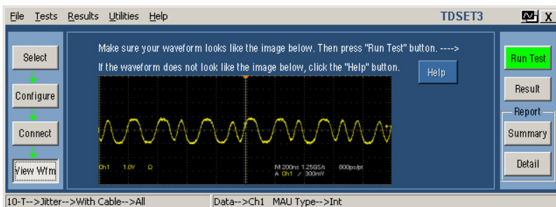
Figure 13- 4: 10BASE-T View Waveform for Jitter with cable
