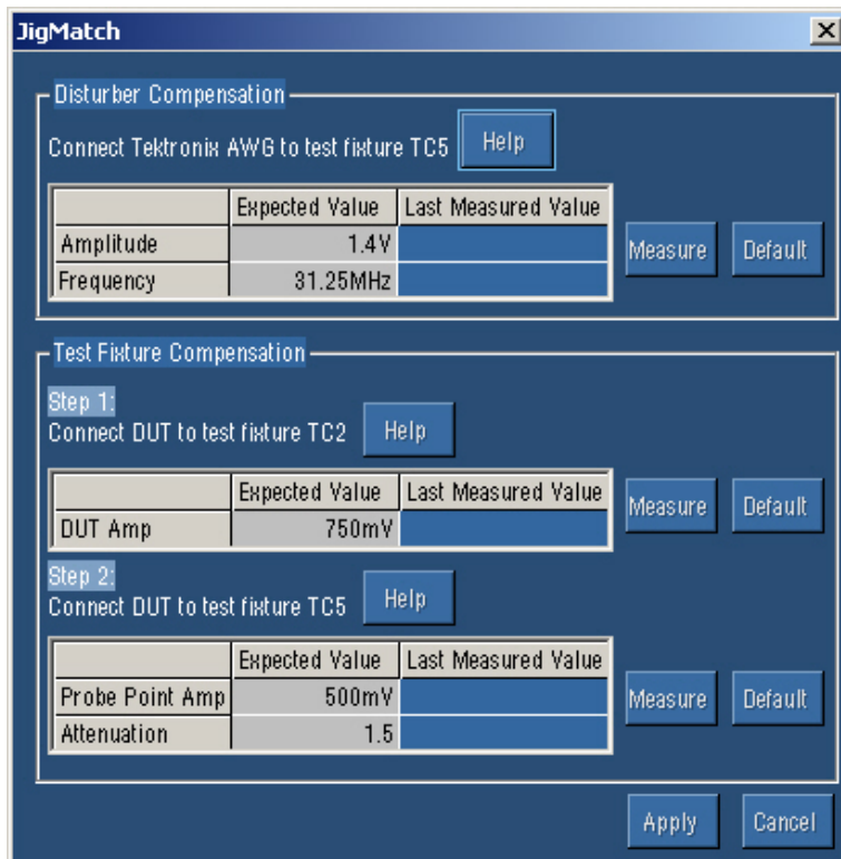
Figure 3-26: Jig Match dialog box
