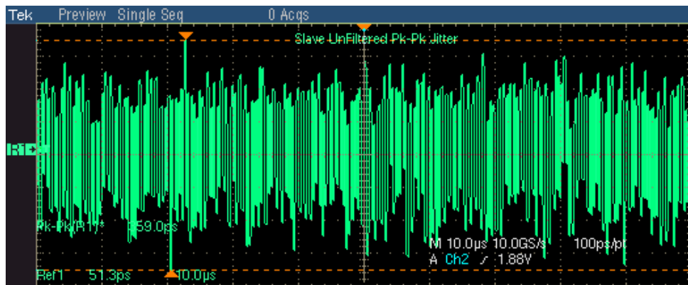
Figure 8-17: TIE Waveform for 100BASE-T Jitter Slave Unfiltered
