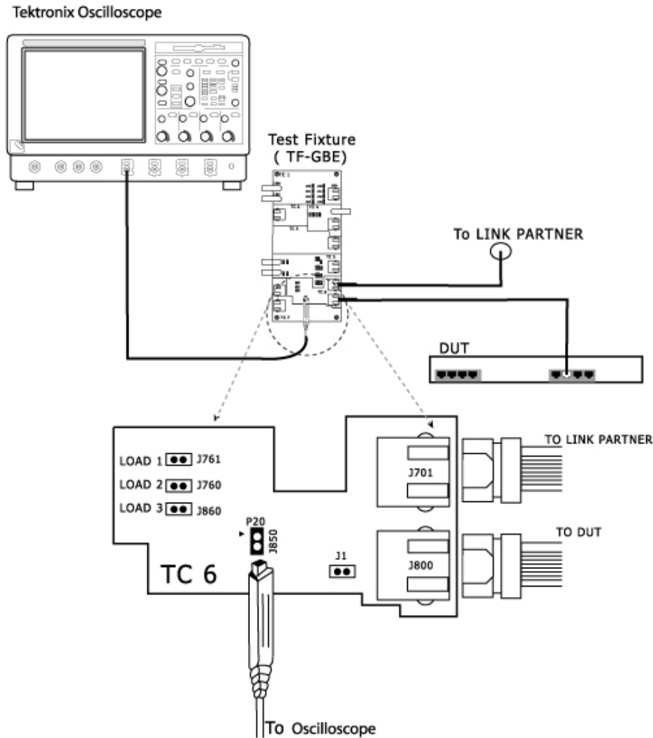
Figure 6-22: 10BASE-T Connections for TP_IDL without Twisted-pair model
