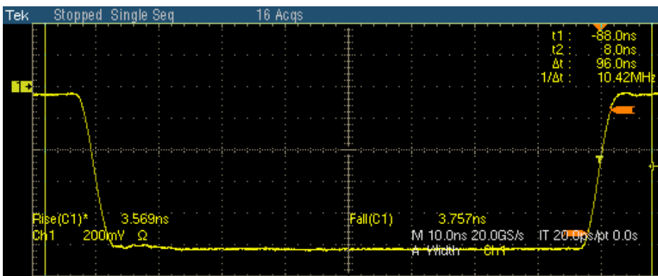
Figure 9-12: Waveform for 100BASE-TX Rise/Fall Time Symmetry for Negative polarity
