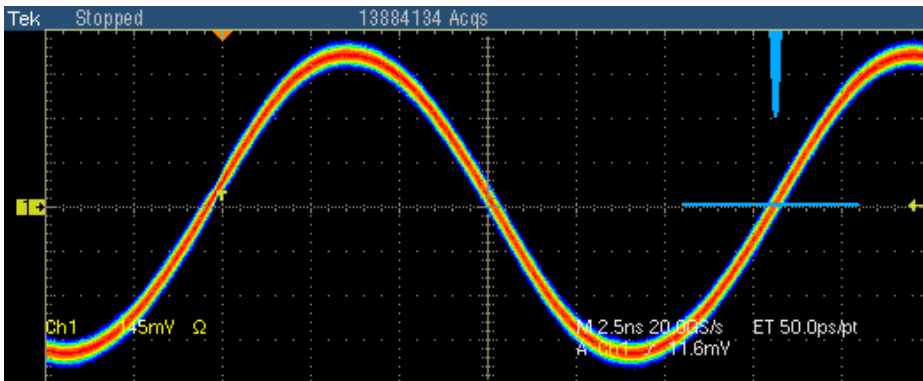
Figure 8-20: Histogram Waveform for 100BASE-T Jitter Slave Unfiltered
