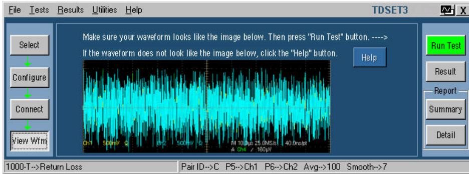
Figure 11- 12: 1000BASE- T View Waveform for Return Loss
