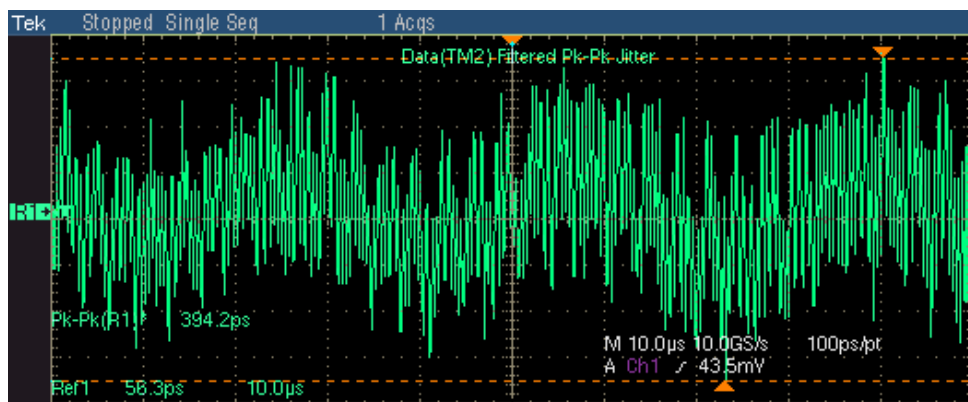
Figure 8-8: 100BASE-T Jitter Master Filtered (without TX_TCLK)
