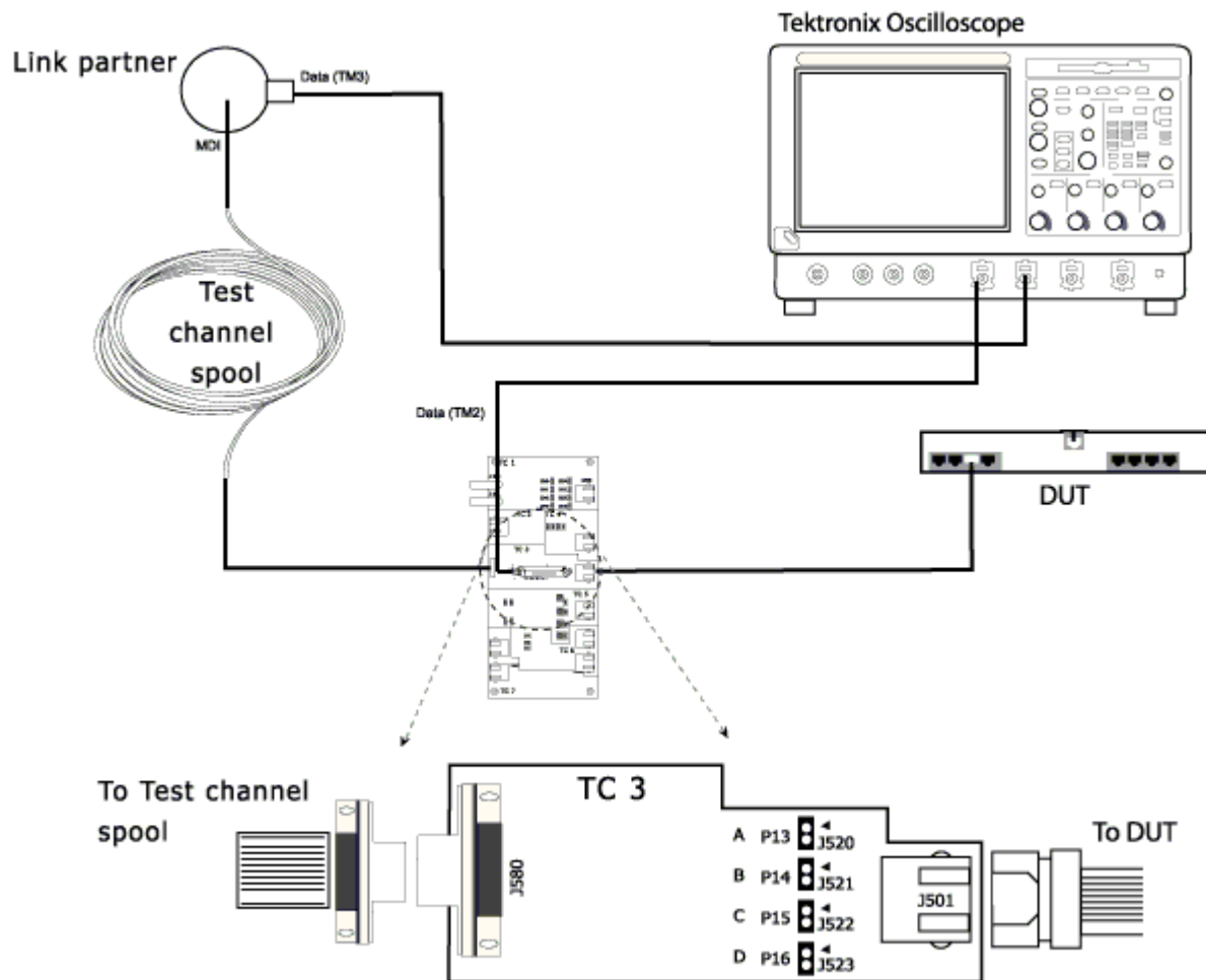
Figure 6-10: 1000BASE-T Connections for Jitter Slave Filtered
