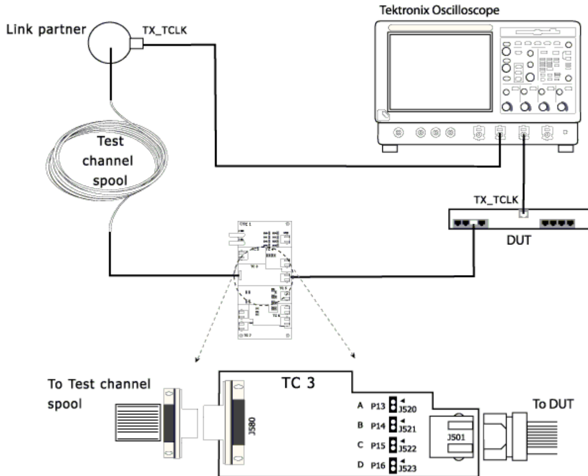
Figure 6-8: 1000BASE-T Step 1 Connections for Jitter Slave Filtered
