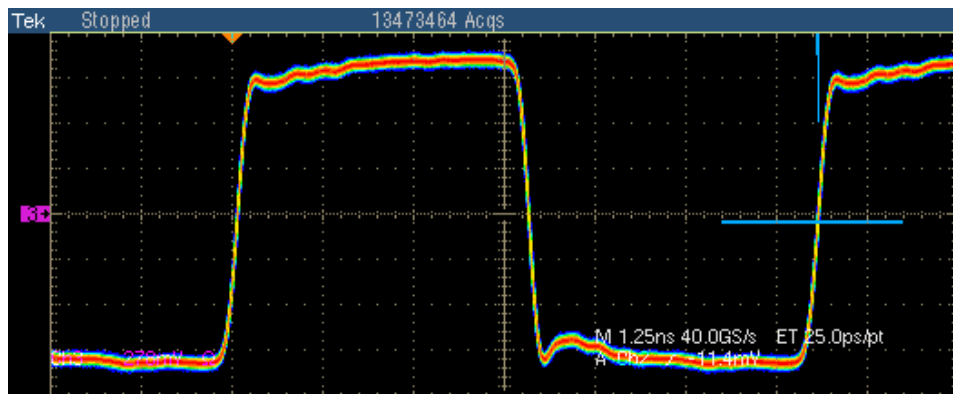
Figure 8-18: Histogram Waveform for 100BASE-T Jitter Slave Unfiltered
